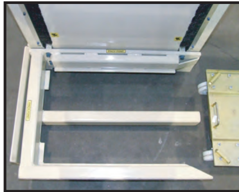
Top view of lift forks
