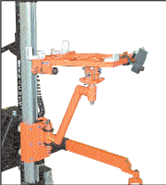
End effector for positioning a fuel tank onto a vehicle.
